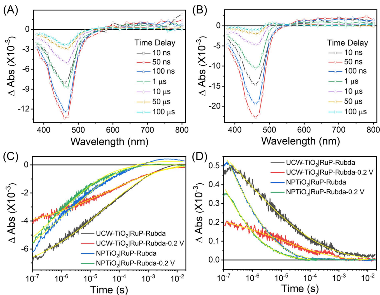
Fig. 7 Full transient absorption spectra at the indicated time delays after pulsed-laser excitation ( \lambda_{\text{ex}} = 532 nm) for the photoelectrodes: (A) UCW-TiO 2 |RuP and (B) NPTiO 2 |RuP. Transient absorption changes measured at 460 nm (C) and 900 nm as a function of delay time, overlaid in yellow are KWW fits. (D) after pulsed-laser excitation ( \lambda_{\text{ex}} = 532 nm) of UCW-TiO 2 |RuP-Rubda (black), NPTiO 2 |RuP-Rubda (blue), UW-TiO 2 |RuP-Rubda (red) and NPTiO 2 |RuP-Rubda (pink) at 0.2 V vs. Ag/AgCl in 0.1 M acetic acid/acetate buffer at pH 4.65 and 0.5 M NaClO 4 .
