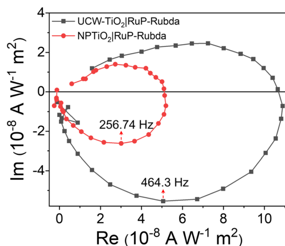
Fig. 8 IMPS responses of UCW-TiO 2 |RuP-Rubda and NPTiO 2 |RuP-Rubda photoanodes.
