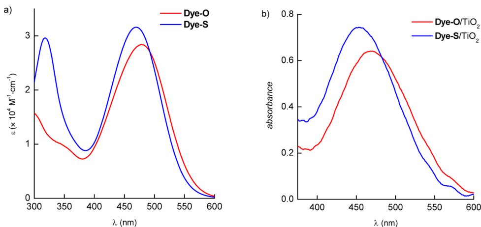
Figure 2. UV–vis absorption spectra of Dye-O (red) and Dye-S (blue) in (a) fluid CH 3 CN solution and (b) anchored to TiO 2 immersed in CH 3 CN solution at 298 K.
