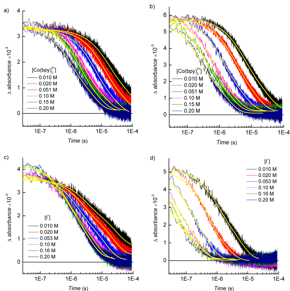
Figure 6. Absorption changes measured after pulsed laser excitation of the sensitized film in the presence of the indicated concentration of [\text{Co}(\text{bpy})_3](\text{ClO}_4)_2 , (a) Dye-O / \text{TiO}_2 and (b) Dye-S / \text{TiO}_2 , or \text{LiI} , (c) Dye-O / \text{TiO}_2 and (d) Dye-S / \text{TiO}_2 in 0.5 M \text{LiClO}_4/\text{CH}_3\text{CN} . Absorbance changes were monitored at a probe wavelength of 635 nm (excitation wavelength, 532 nm; laser fluence, 0.1 \text{ mJ}/\text{cm}^2 ). Overlaid in yellow are the best fits to biexponential kinetic model.
