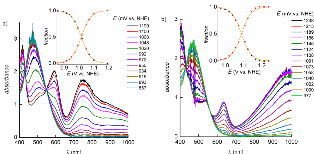
Figure 3. Visible absorption spectra of (a) Dye-O /TiO 2 (dye surface coverage \Gamma = 1.0 \times 10^{-8} mol cm -2 ) and (b) Dye-S /TiO 2 ( \Gamma = 5.3 \times 10^{-8} mol cm -2 ) measured at the indicated applied potentials in 0.5 M LiClO 4 CH 3 CN solution. The insets show the fraction ( x ) of dye molecules present in the reduced (■) and the oxidized state (red ●). Overlaid on this data is a sigmoidal fit, x = 1/(1 + 10 \exp((E_{\text{app}} - E^\circ_{1/2})/a \times 59 \text{ mV})) , where a is the ideality factor determined to be 1.27 for Dye-O /TiO 2 and 1.05 for Dye-S /TiO 2 .
