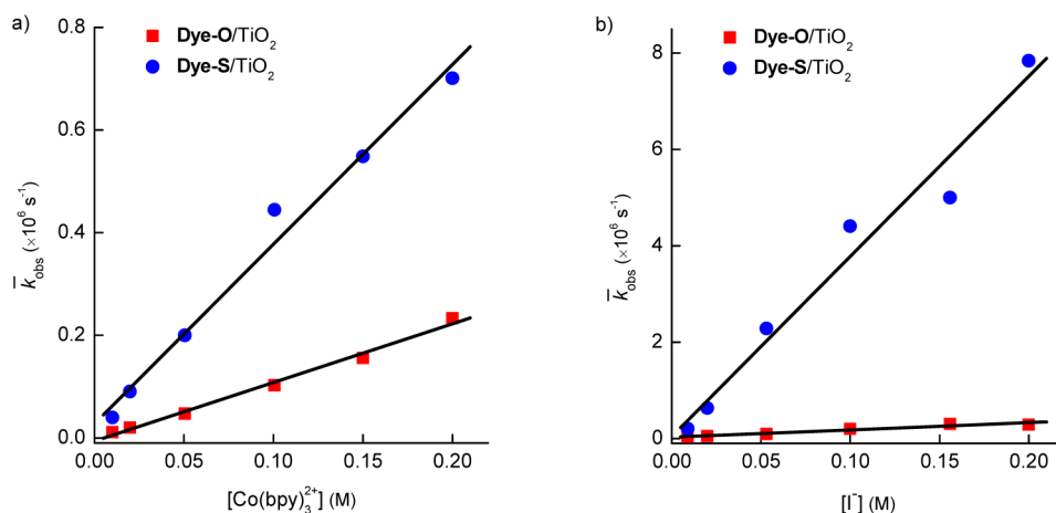
Figure 7. Plots of observed regeneration rate constants ( \bar{k}_{\text{obs}} ) of Dye-O / \text{TiO}_2 (red ■) and Dye-S / \text{TiO}_2 (blue ●) obtained from the kinetics fits versus titrated (a) [\text{Co}(\text{bpy})_3]^{2+} and (b) [\text{I}^-] concentrations.
